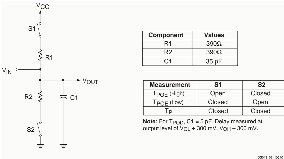
Figure 3: AC Load Circuit
