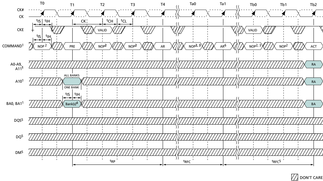
Figure 47: Auto Refresh Mode
