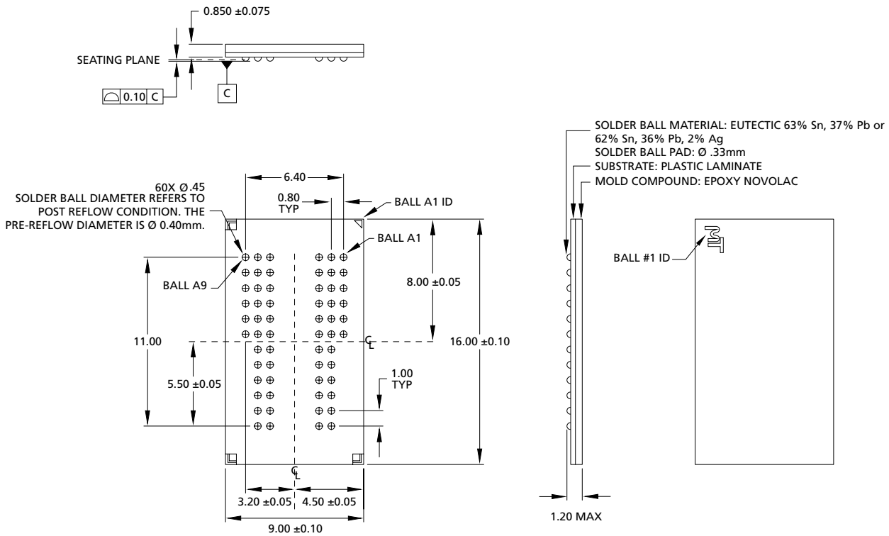
Figure 55: 60-Ball FBGA (16 x 9mm)
