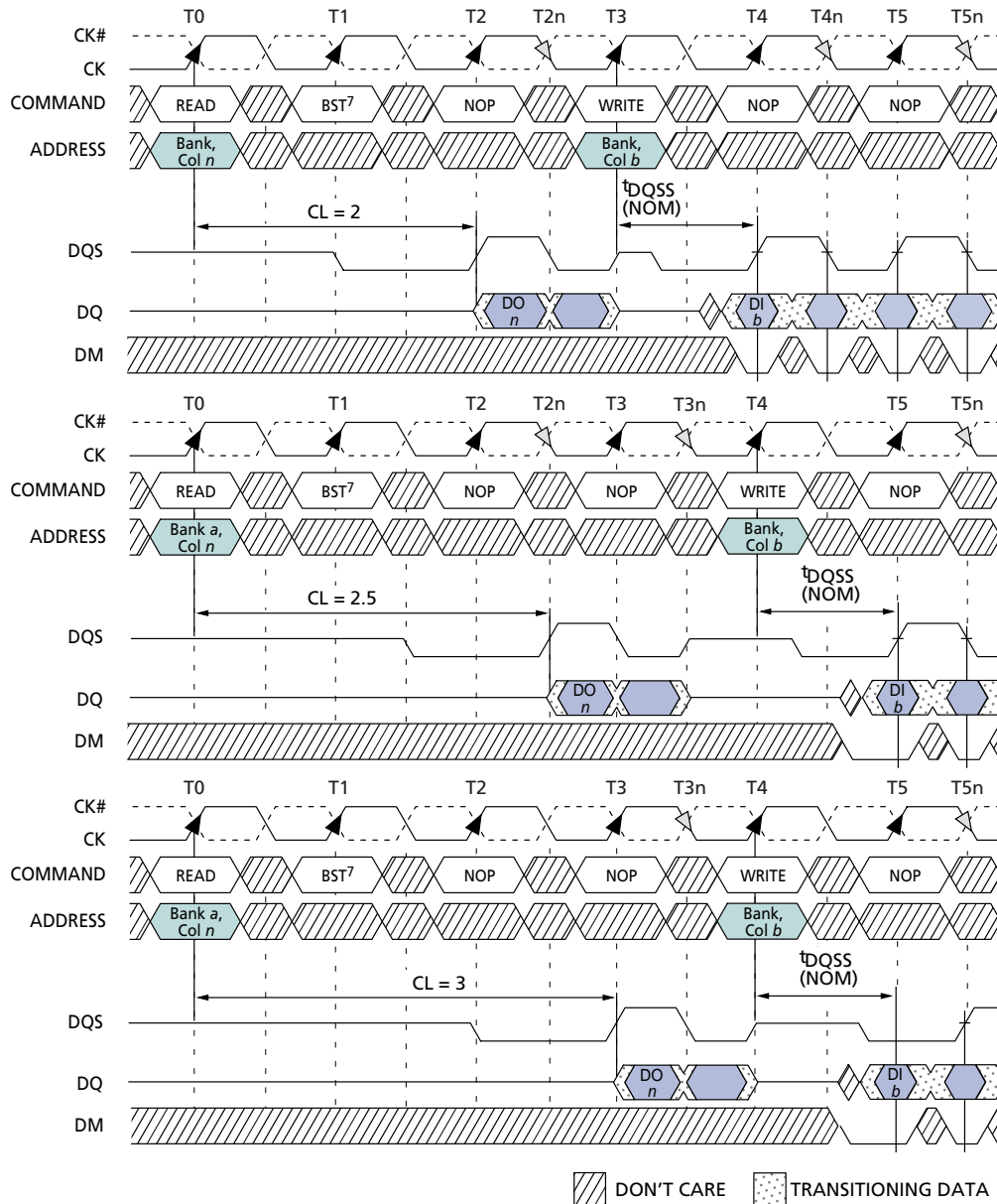
Figure 18: READ to WRITE
