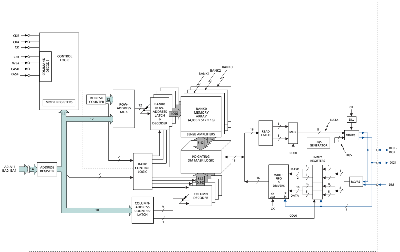
Figure 4: Functional Block Diagram 16 Meg x 8
