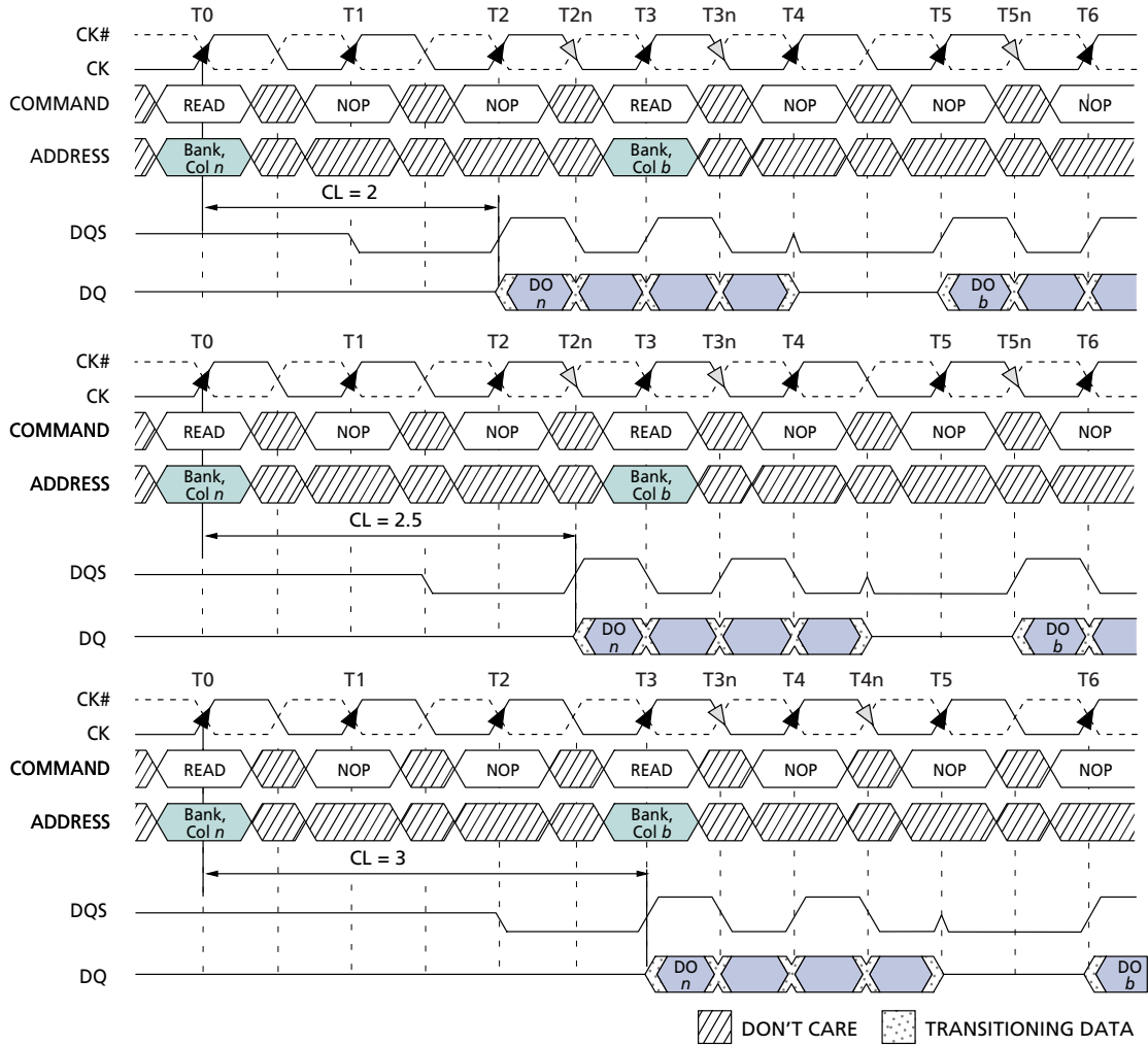
Figure 15: Nonconsecutive READ Bursts
