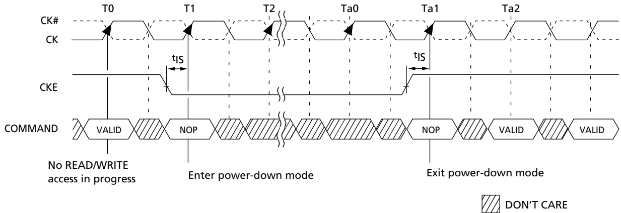
Figure 32: Power-Down
