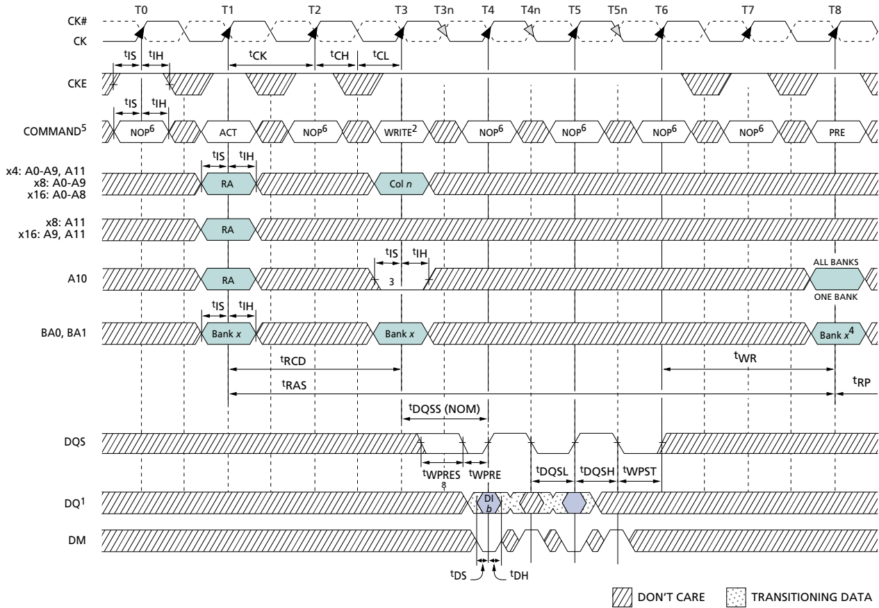
Figure 53: Write - DM Operation
