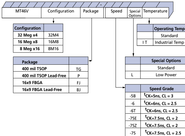
Figure 2: 128Mb DDR SDRAM Part Numbers
