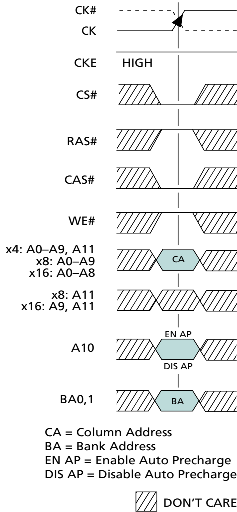
Figure 12: READ Command
