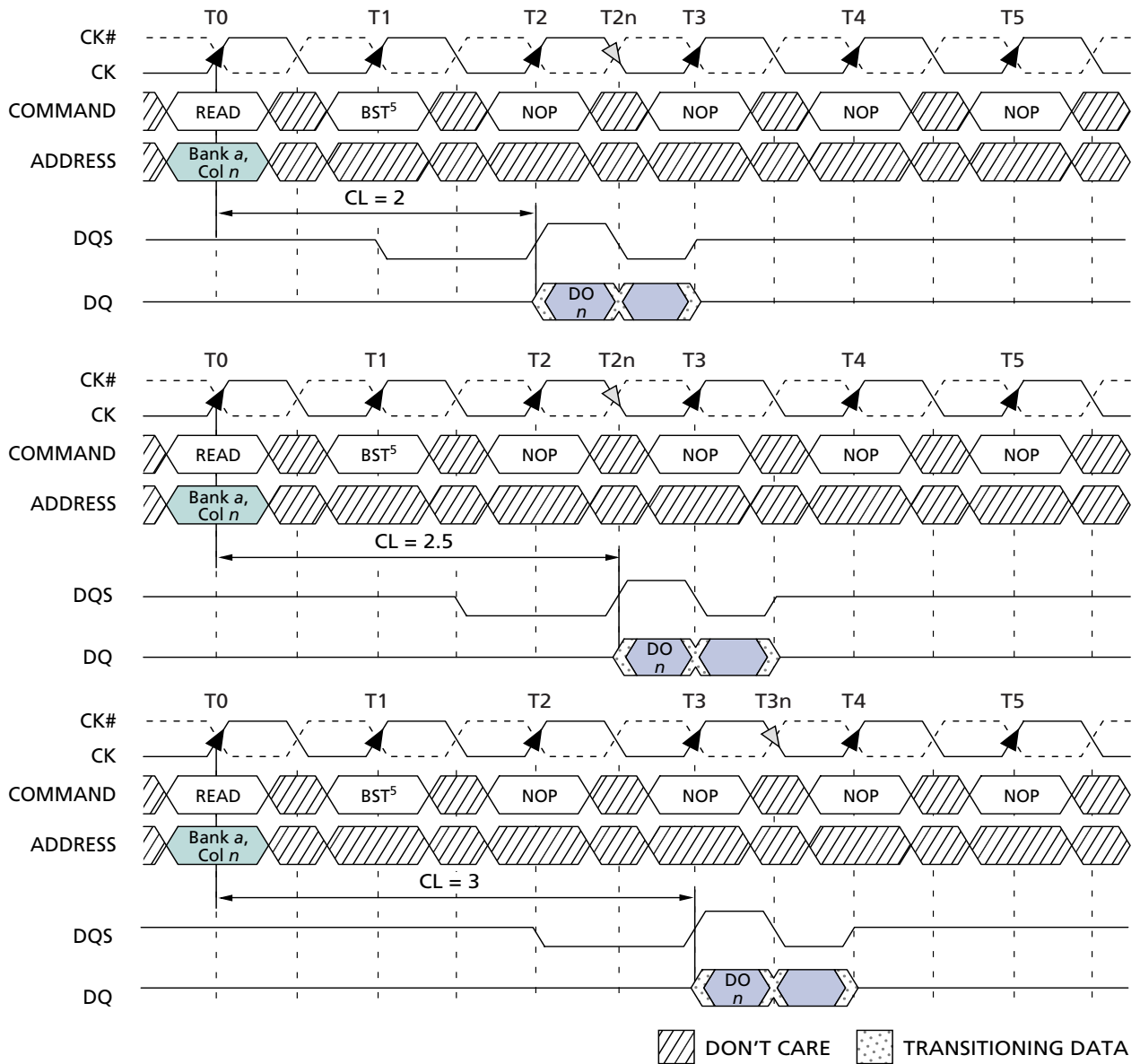
Figure 17: Terminating a READ Burst
