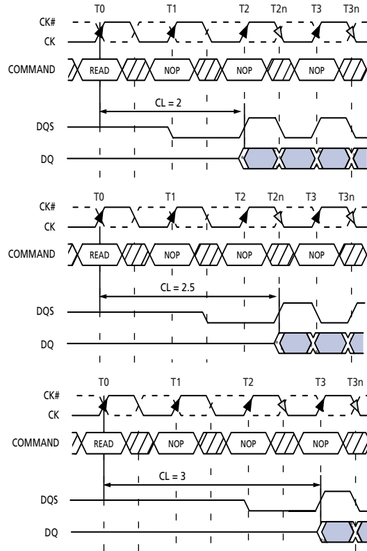
Figure 8: CAS Latency
