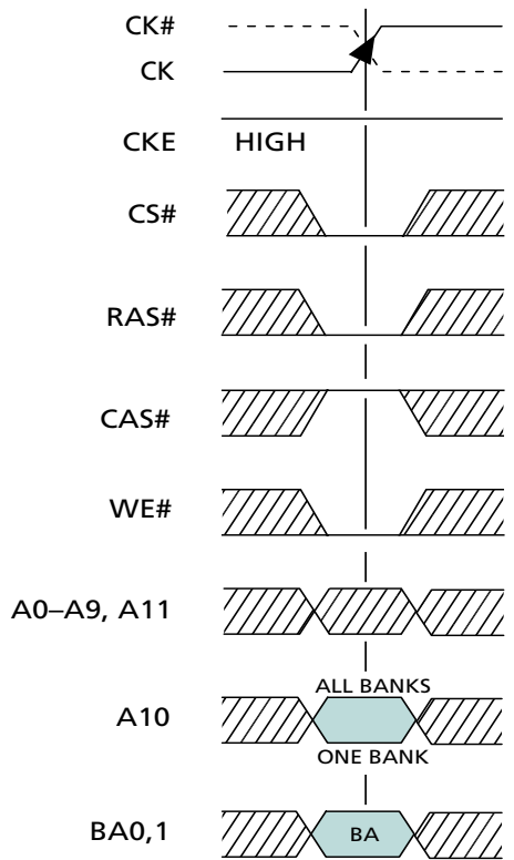
Figure 31: PRECHARGE Command
