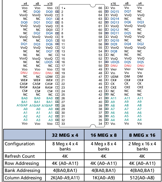
Figure 1: Pin Assignment (Top View) 66-pin TSOP
