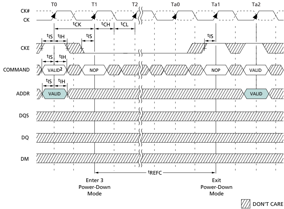
Figure 46: Power-Down Mode
