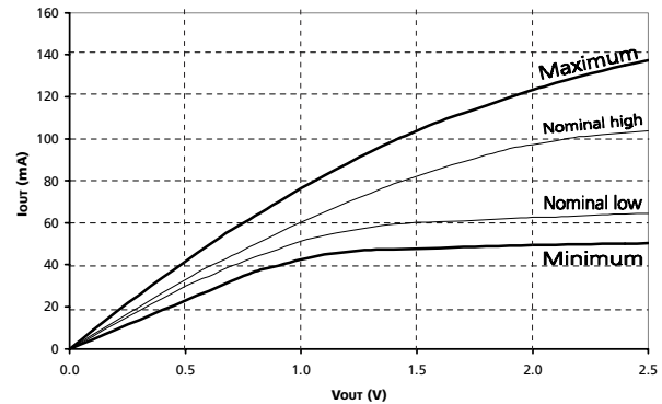
Figure 37: Full Drive Pull-Up Characteristics
