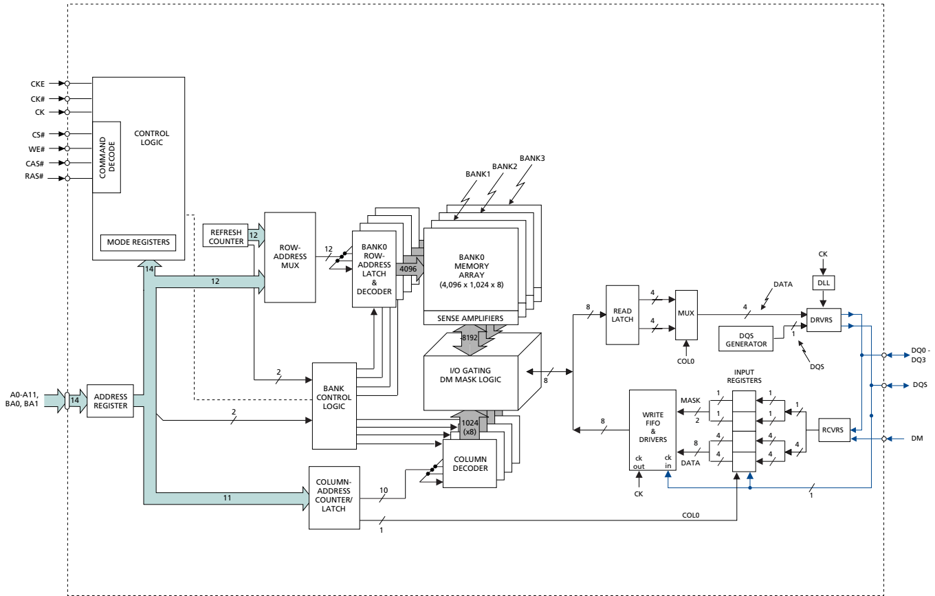
Figure 3: Functional Block Diagram 32 Meg x 4
