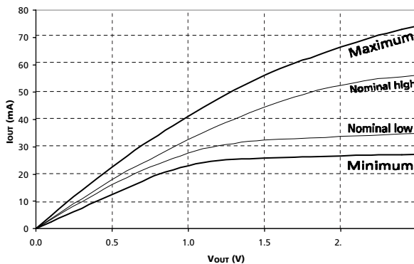
Figure 39: Reduced Drive Pull-Up Characteristics
