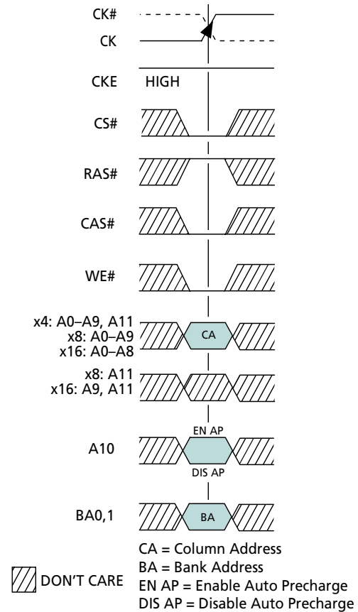
Figure 20: WRITE Command
