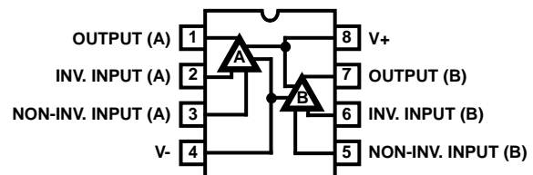
CA1458, CA1558, LM1458 (PDIP) TOP VIEW
