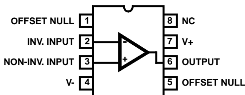
CA741, CA741C, LM741, LM741C (PDIP) TOP VIEW
