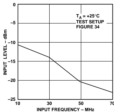
Figure 37. 1 dB Compression Point, -10 dB/+30 dB Mode, Gain = 30 dB
