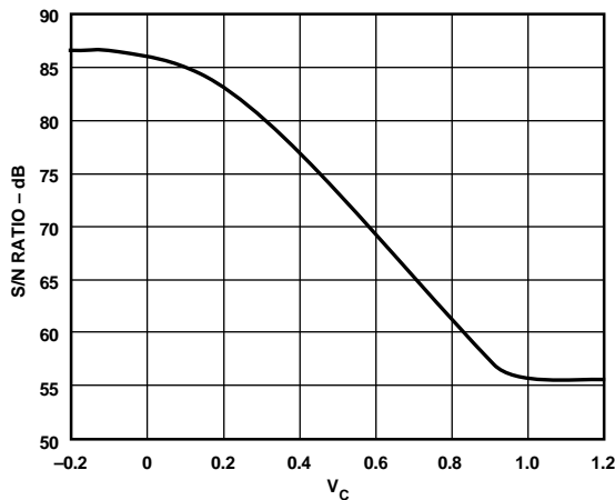
Figure 14. SNR vs. Control Voltage—Low Ripple Mode
